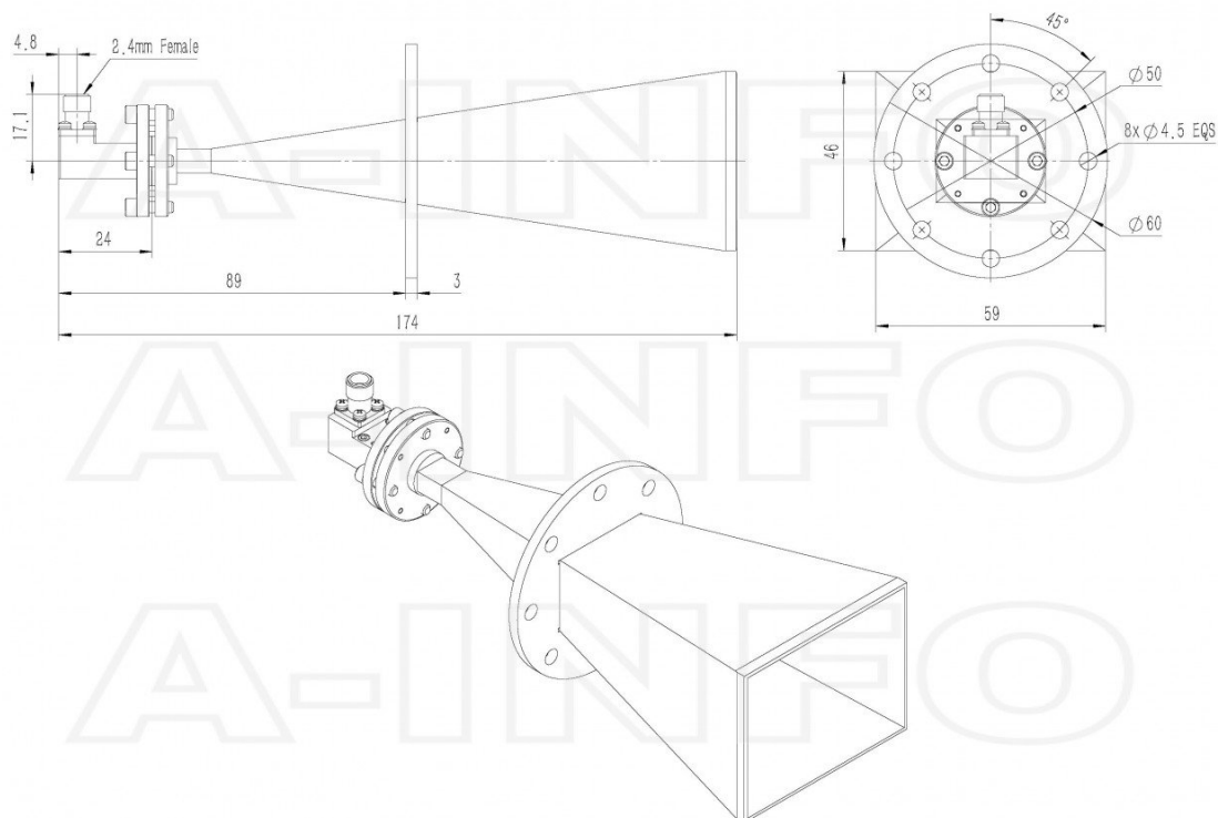
2.4mm-Female Output (P/N: LB-22-25-C2-2.4F)
