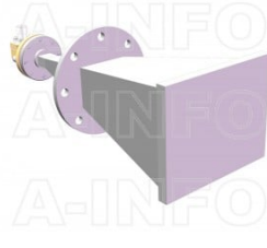
LB-22-25-C2-2.4FSPO Standard Gain Horn Antenna 33-50GHz 25dB Gain 2.4mm Female
